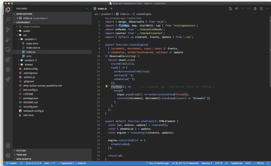
Figure 2: Visual Studio Code after navigating cursor to the flatMap operator on Line 18.
