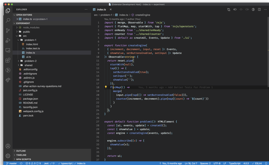
Figure 3: Visual Studio Code indicating available code actions on Line 18 using a yellow light bulb icon.
