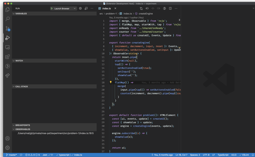
Figure 6: Visual Studio Code showing the debugging view after launching “Problem 1.”
