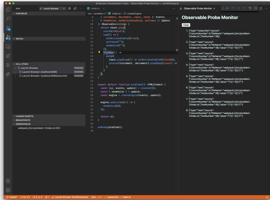
Figure 8: Visual Studio Code showing live telemetry in the “Observable Probe Monitor.”
