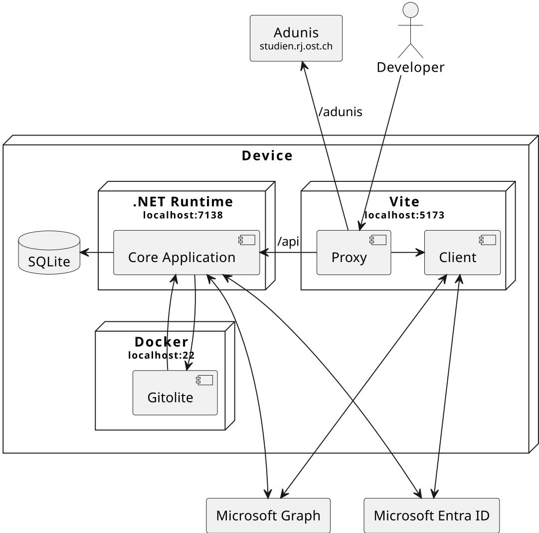
Figure 14: The deployment of the system when working locally
