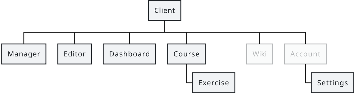
Figure 6: The sitemap of the Client single-page application
