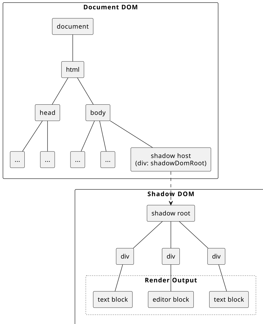
Figure 17: Encapsulation of render output using shadow DOM
