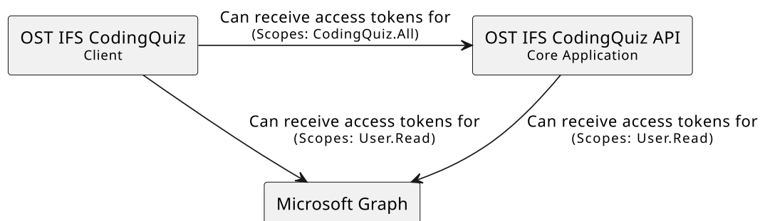
Figure 19: An overview of the Microsoft Entra ID access token scopes
