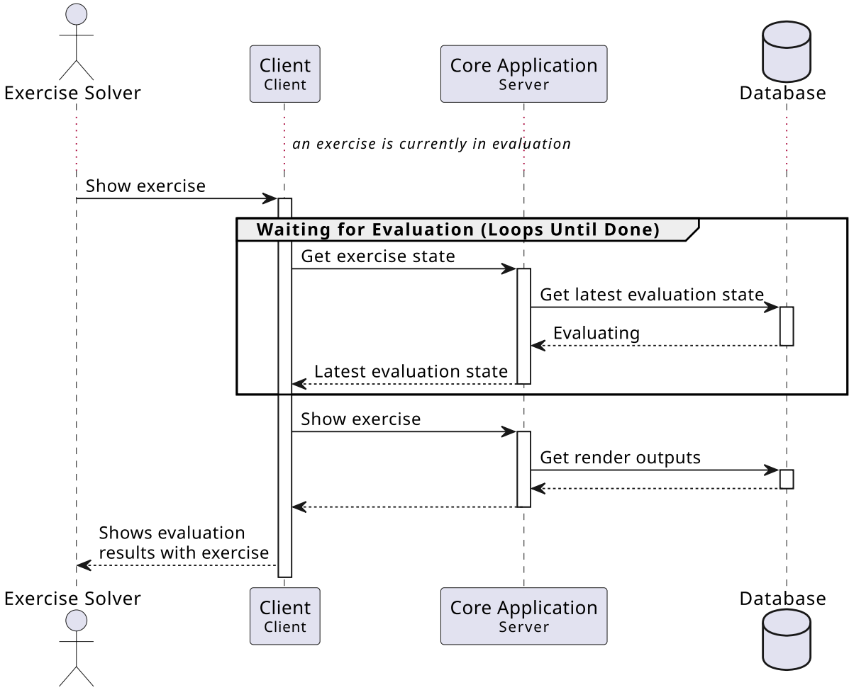
Figure 11: The process when waiting for evaluation
