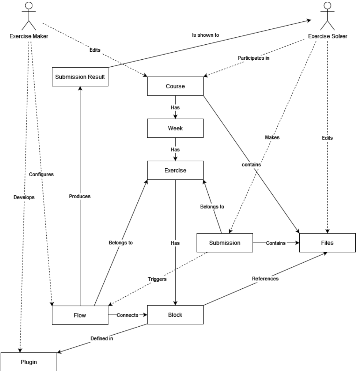
Figure 16: The conceptual domain model of the system
