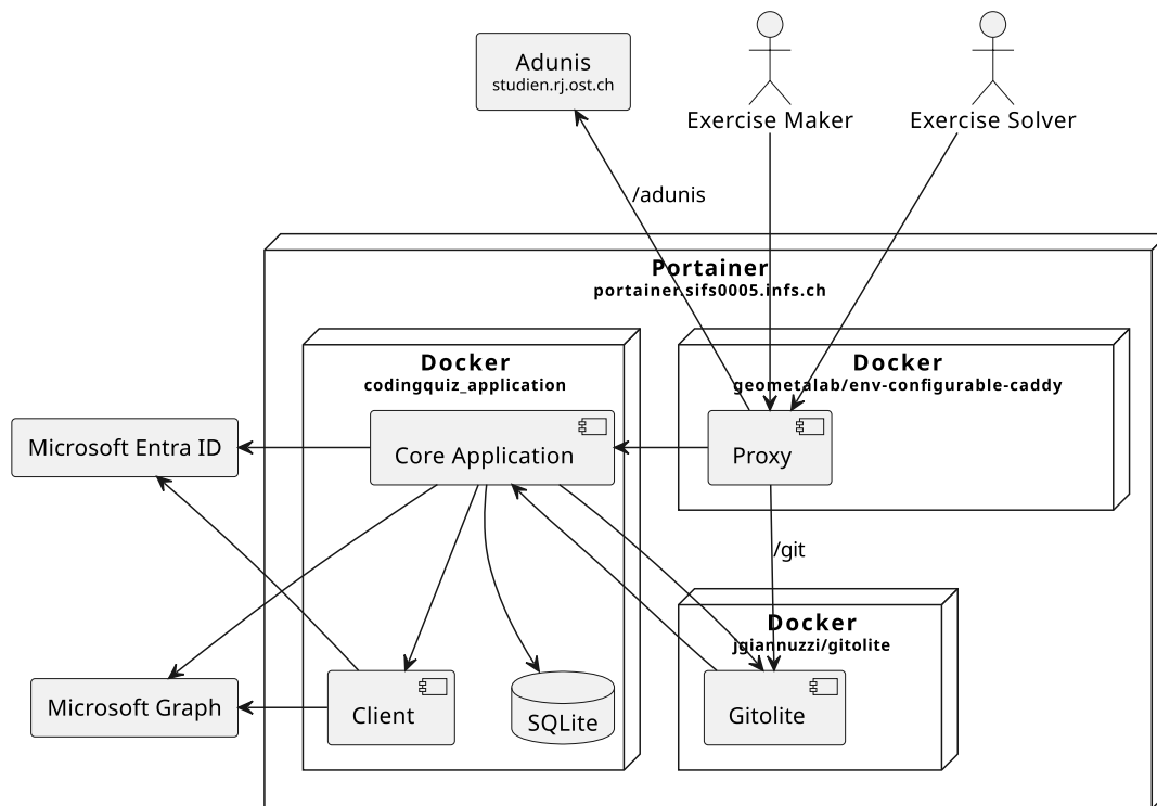
Figure 15: The deployment of the system on the OST Portainer instance
