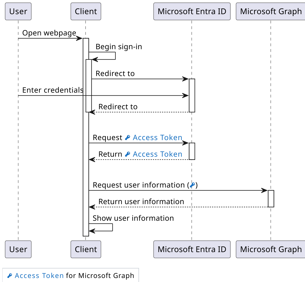
Figure 12: The sign-in process of the system
