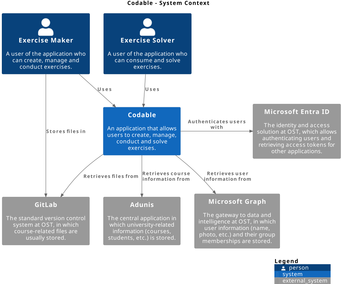
Figure 4: An overview of the scope and context of the application
