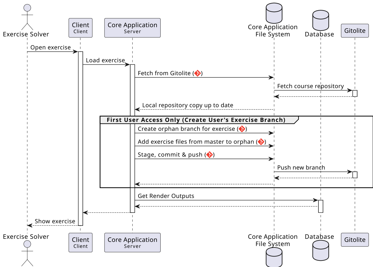
Figure 8: The process when opening an exercise
