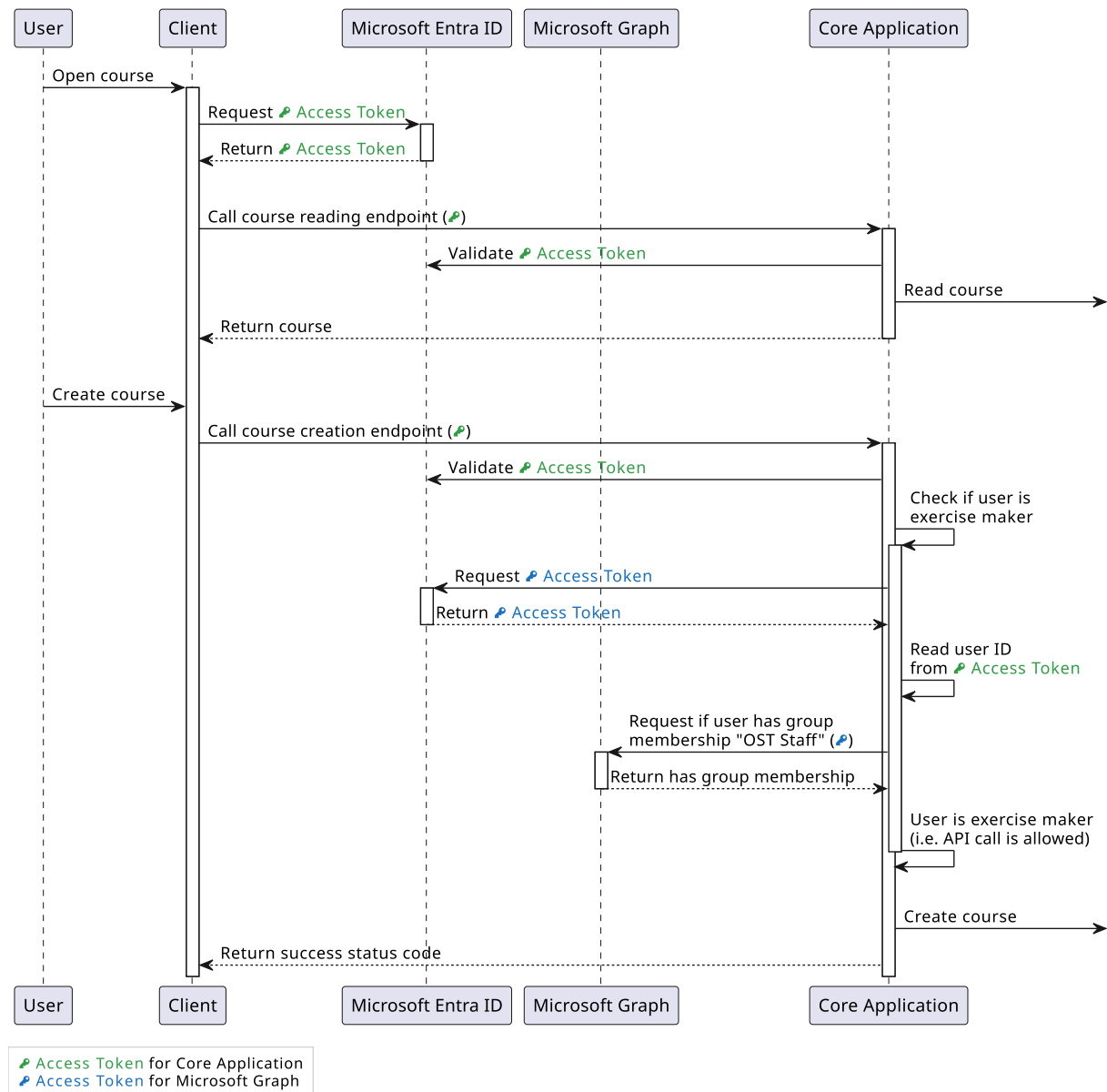
Figure 13: The authorization process when calling API endpoints
