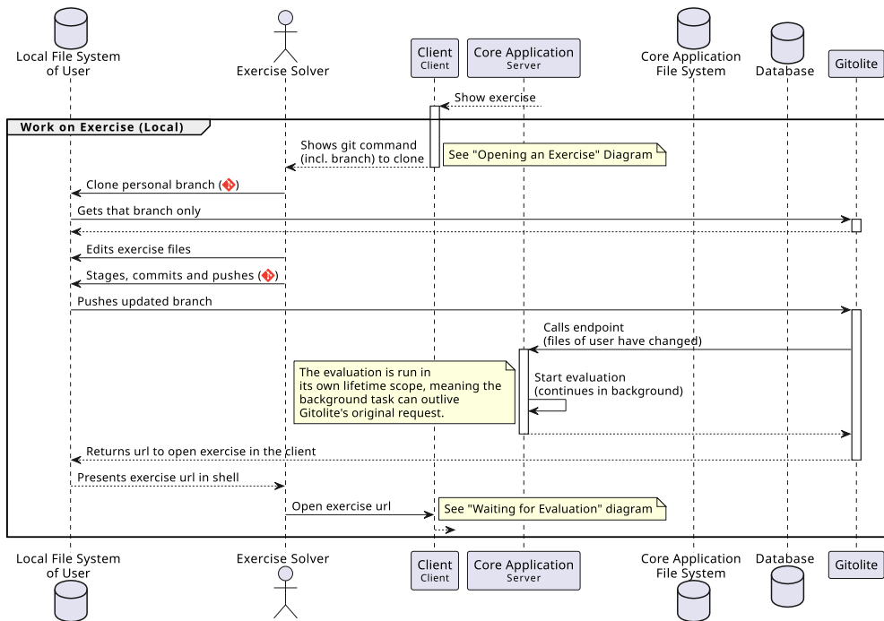
Figure 10: The process when editing an exercise locally
