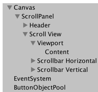
Figure 30: Scrollable List Hierarchy
